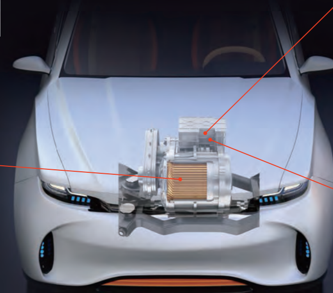
Leaf springs for cooling HEV and EV elements These spring hold semiconductors to heat sink with the force of spring.
