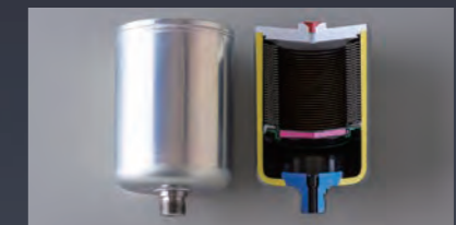
Accumulators Designing an energy-saving system for HEV vehicle brakes
