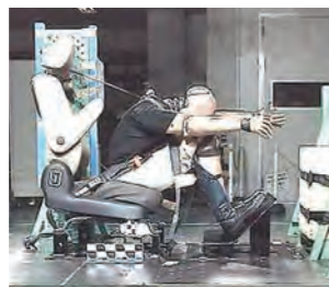
Safety evaluation for seats through hydraulic sled tests
