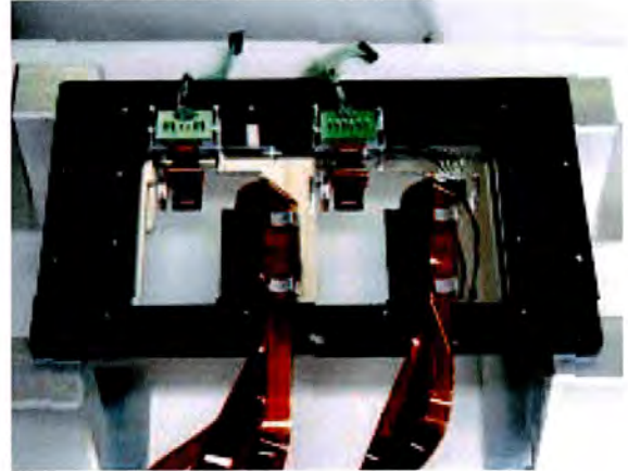
Multi-tip contacting unit
