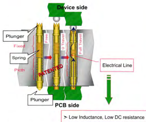
Thermal Socket Design
